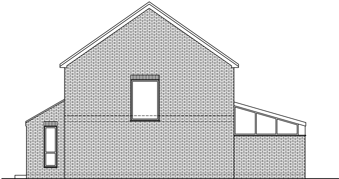
Pre-existing Right Side Elevation Scale: 1/100
