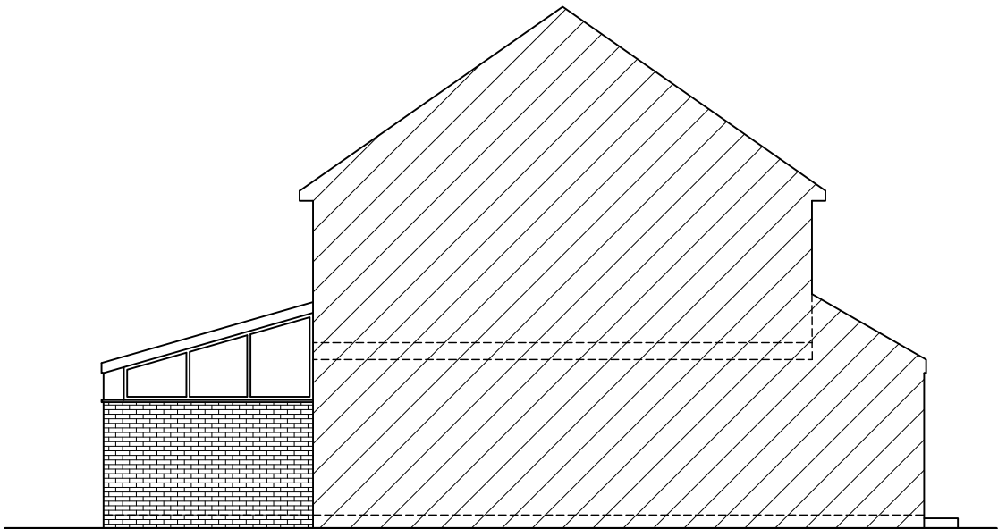
Pre-existing Left Side Elevation Scale: 1/100
