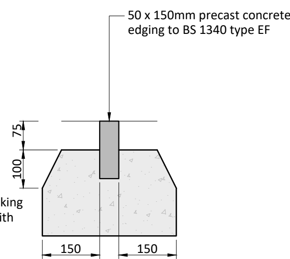
Kerb Detail 4 - EF (Scale 1:10)
