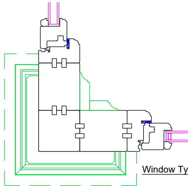
PLAN VIEW OF LARGE CORNER PILASTER
