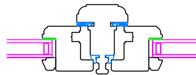
Window Mullion
