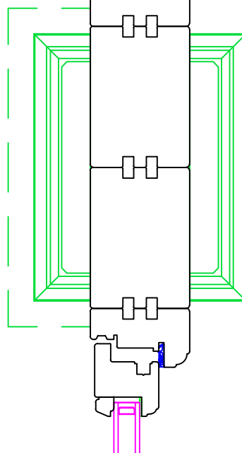
PLAN VIEW OF LARGE IN-LINE PILASTER
