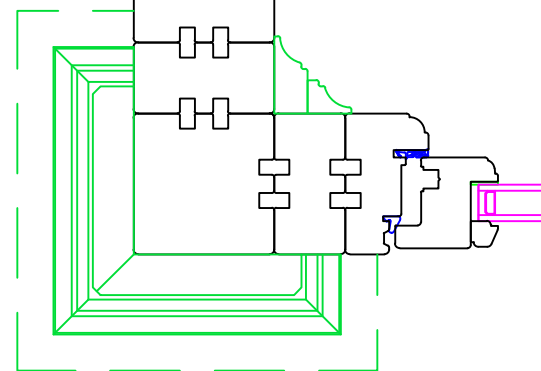
PLAN VIEW OF STD CORNER PILASTER
