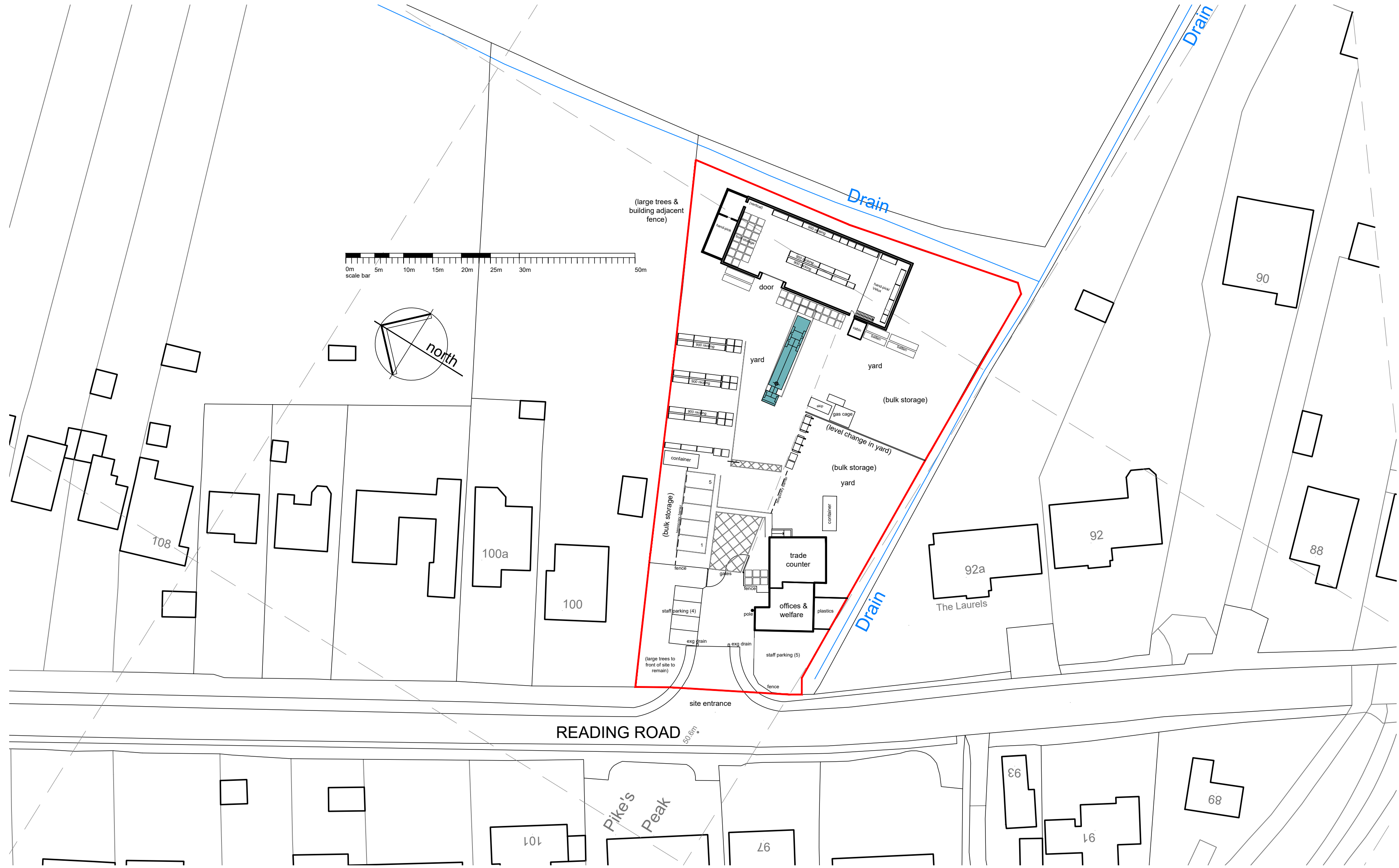
SITE BLOCK PLAN (1:500)
