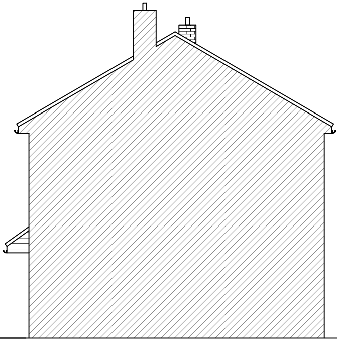
Proposed Side Elevation - A
