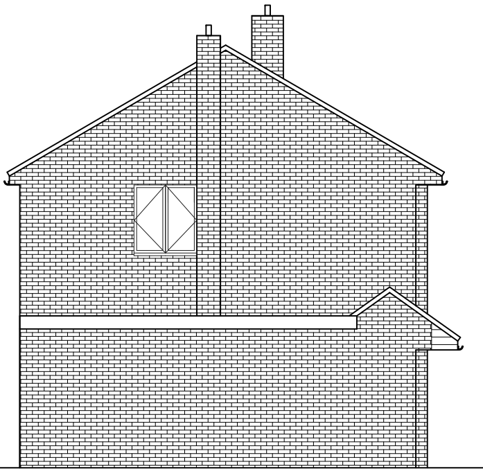
Proposed Side Elevation - B
