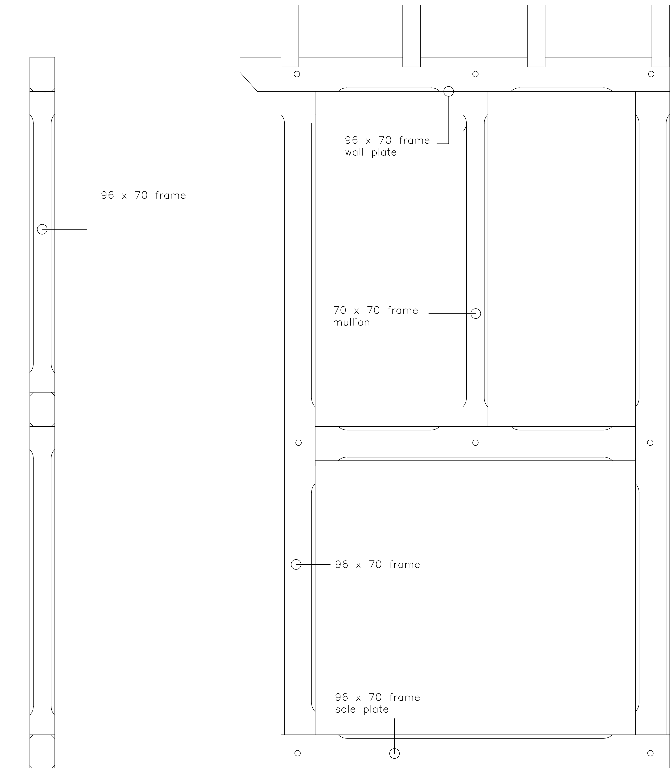
PORCH VERTICAL FRAME SECTION INTERNAL PORCH FRAME ELEVATION
