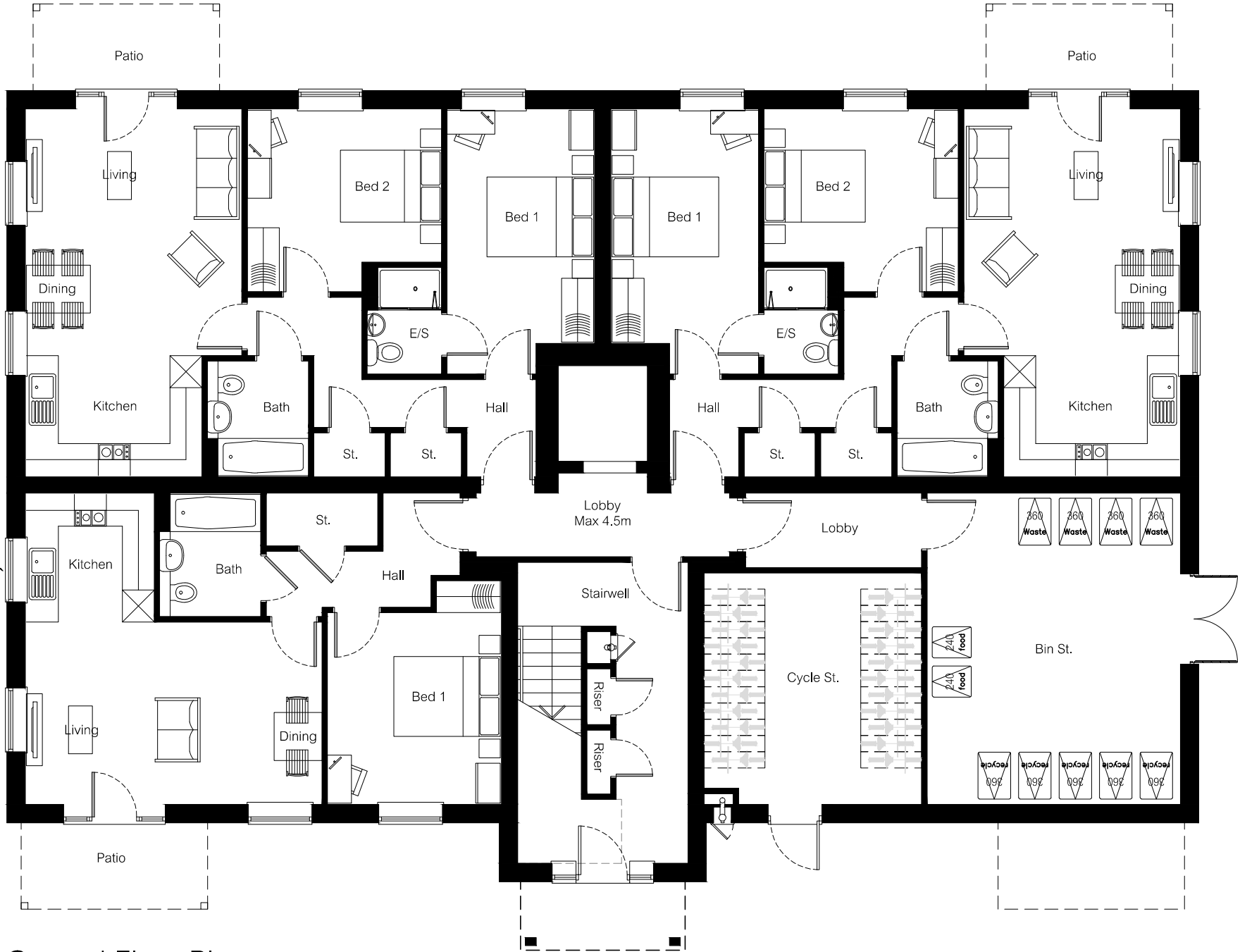
Ground Floor Plan ^ - Lower Panel Blocked Up Internally
