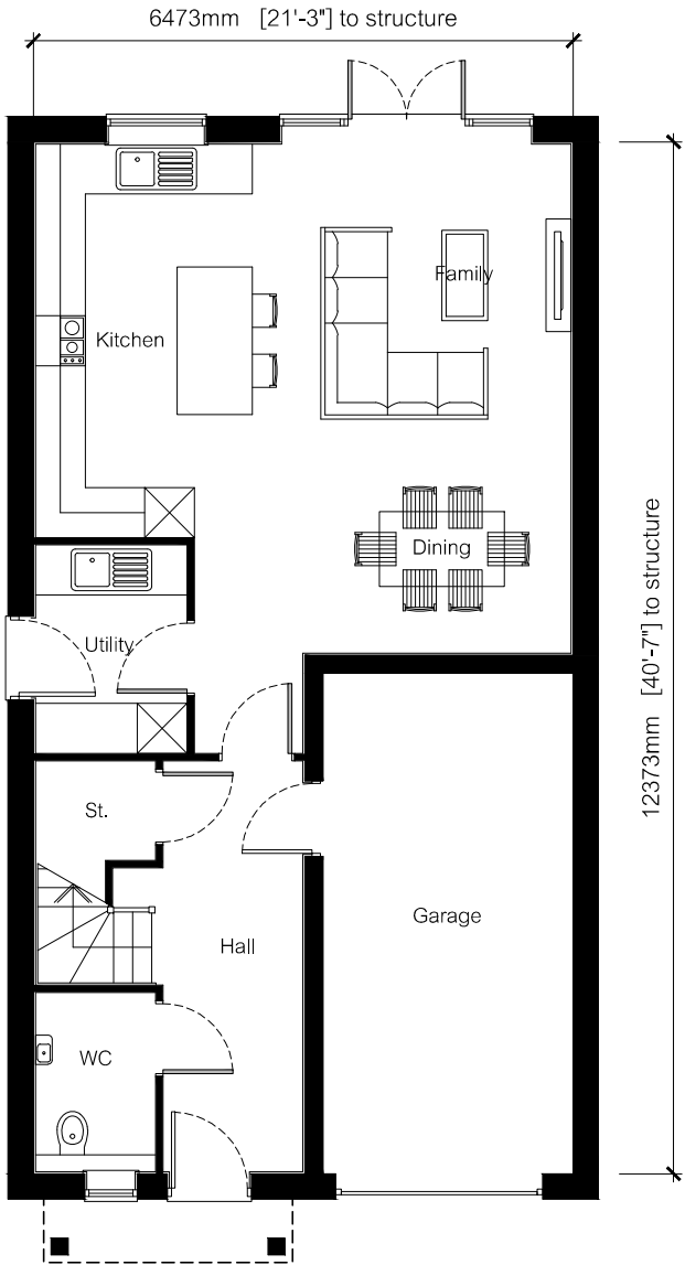
Ground Floor Plan Plot 50
