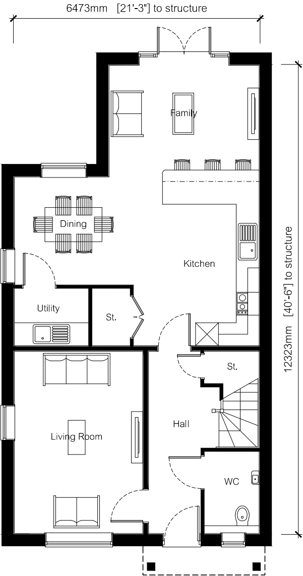
Ground Floor Plan Plot 51
