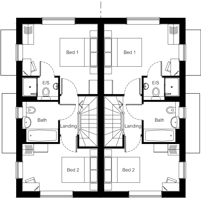
HT 2A Plot 53 HT 2A Plot 52 First Floor
