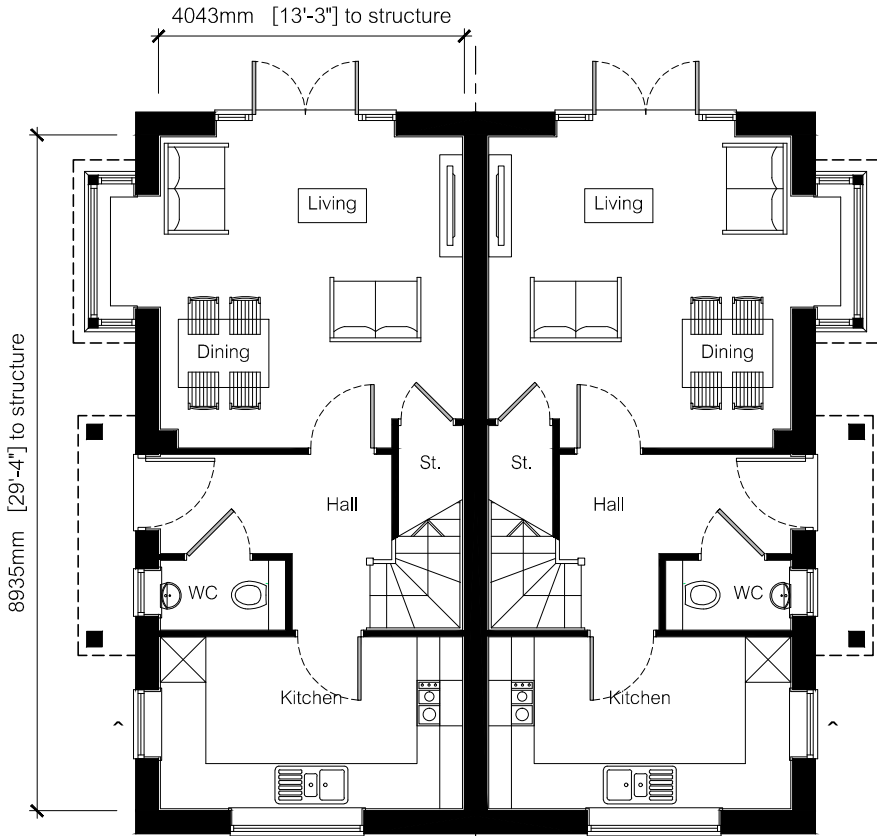
HT 2A Plot 53 HT 2A Plot 52 Ground Floor ^ - Lower Panel Blocked Up Internally
