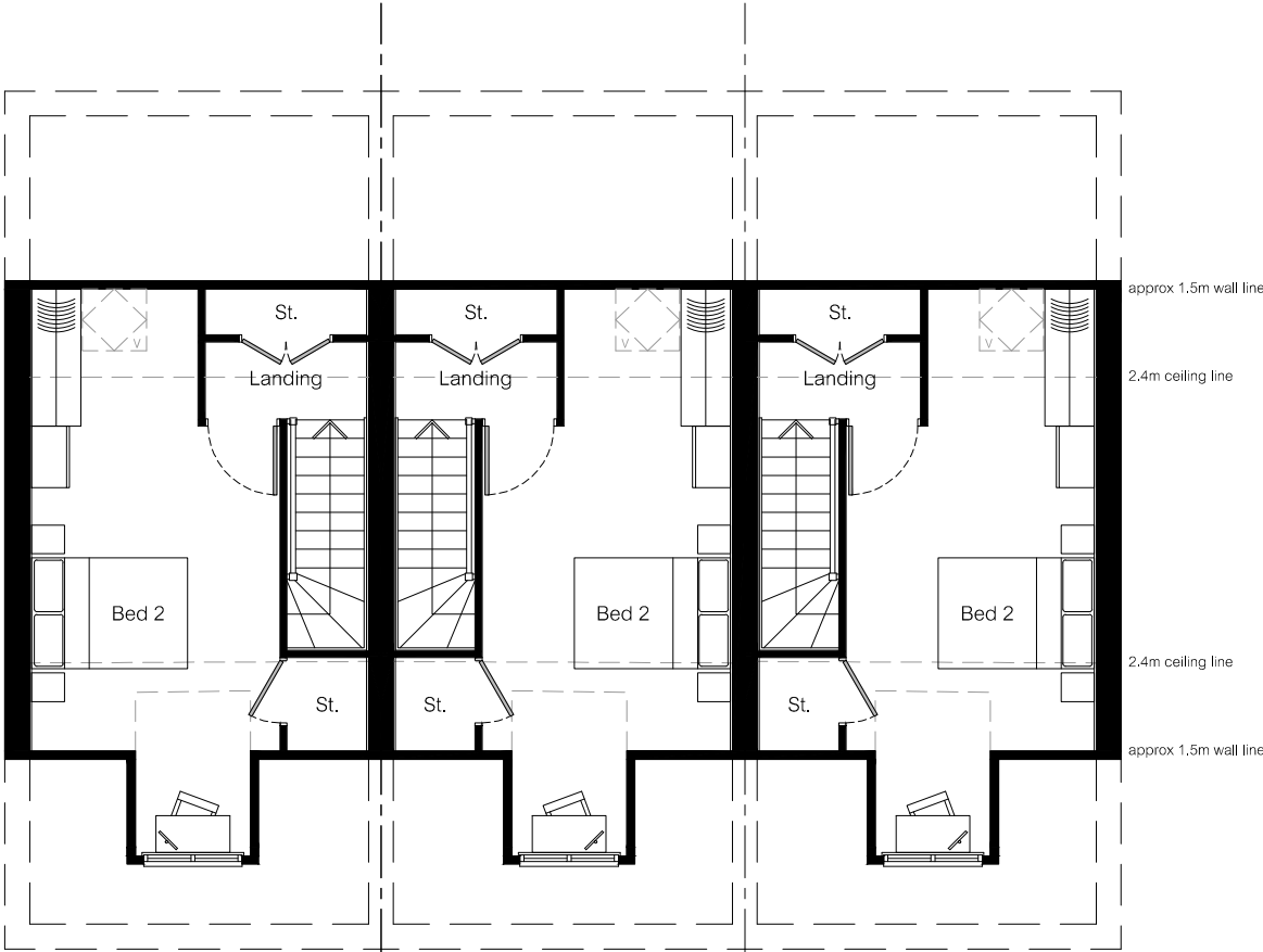
HT 3AA Plot 27 Second Floor
