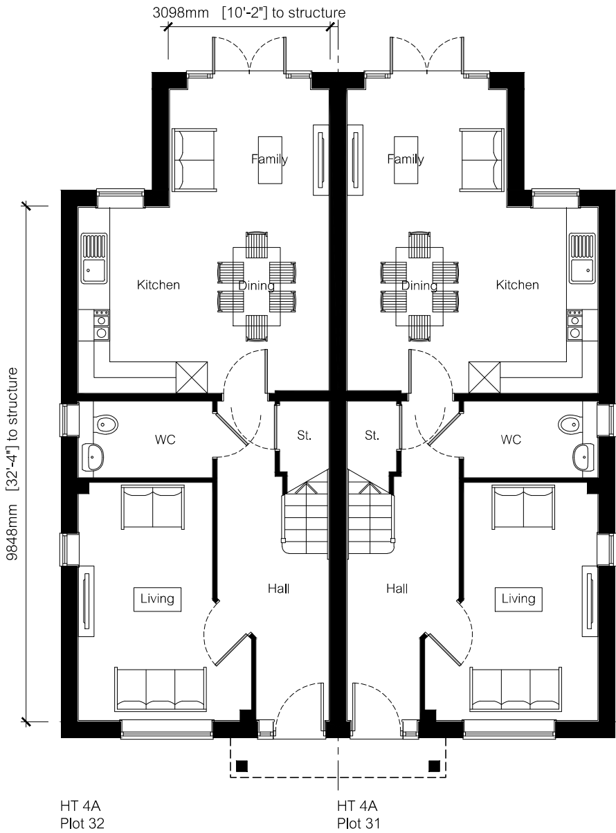
Ground Floor
