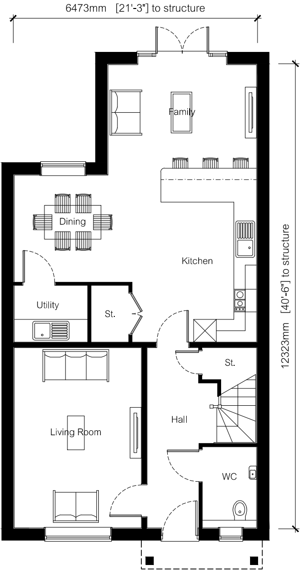
Ground Floor Plan Plot 33
