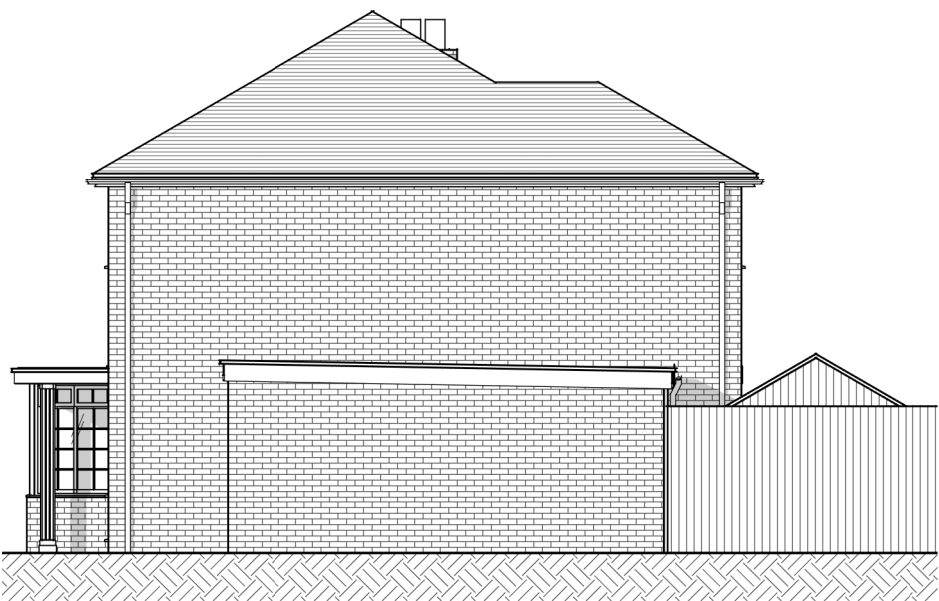
Existing Elevation General Arrangement | Scale 1 : 100
