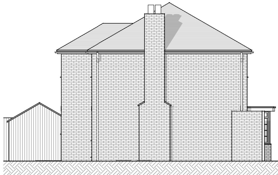
Existing Elevation General Arrangement | Scale 1 : 100
