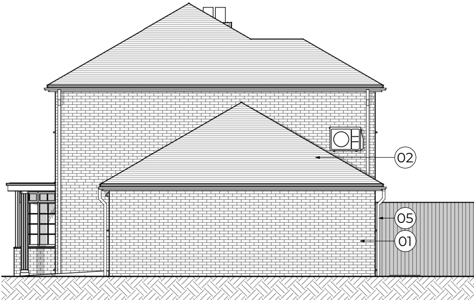
Proposed Elevation General Arrangement | Scale 1 : 100
