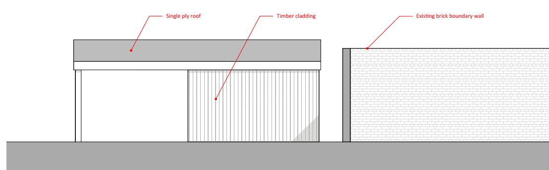
West Elevation 1:100
