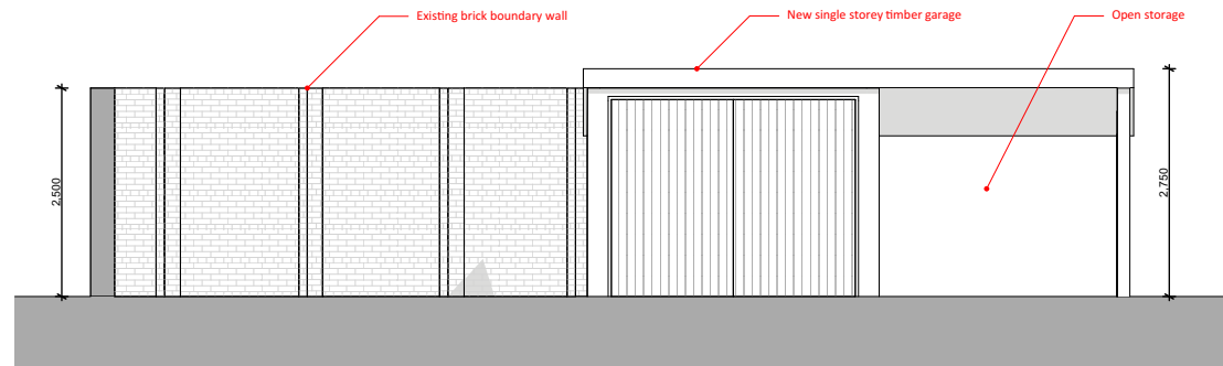
East Elevation 1:100
