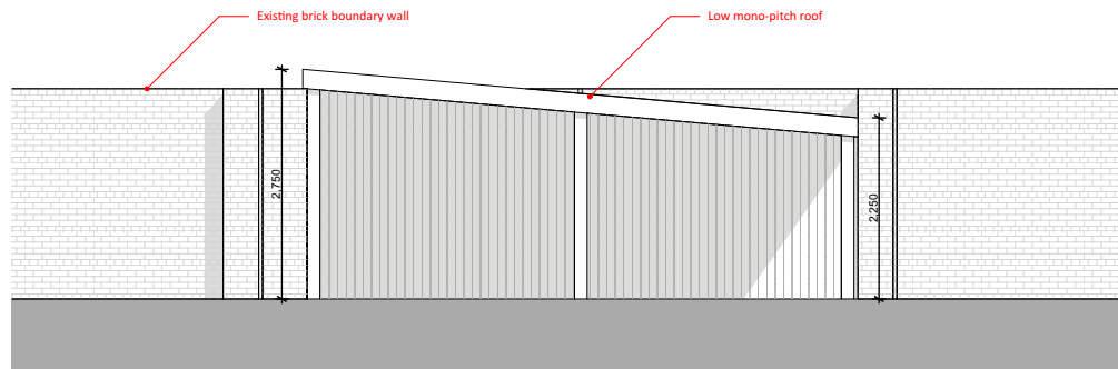
North Elevation 1:100
