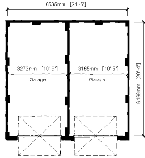
Plan Variation - 1:200
