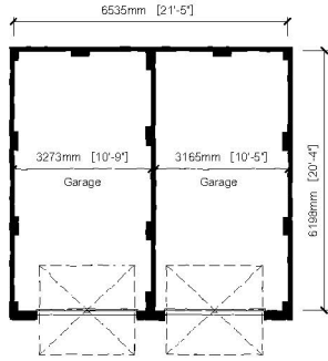
Plan Variation - 1:200
