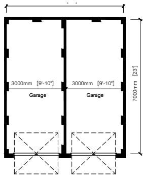
Plan Variation - 1:200
