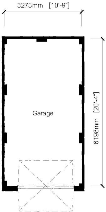
Floor Plan
