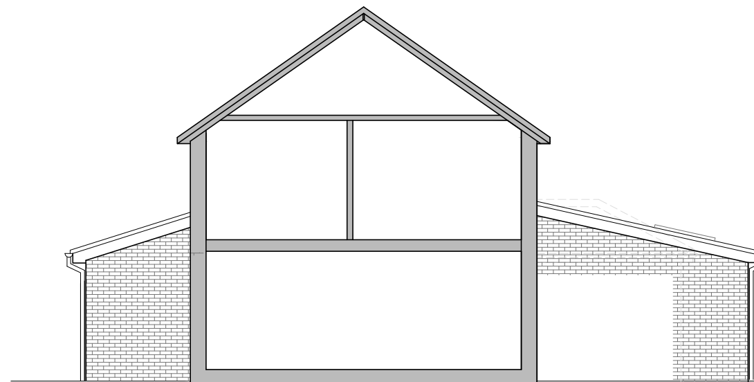
Side Elevation
