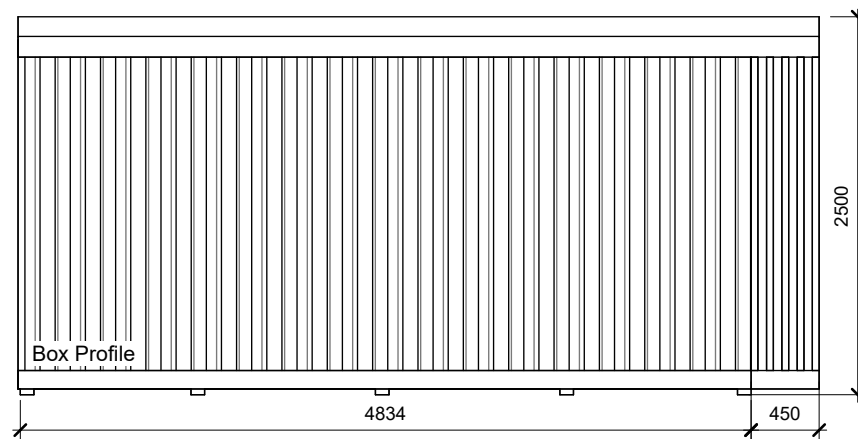
3 Rear Elevation 1 : 50
