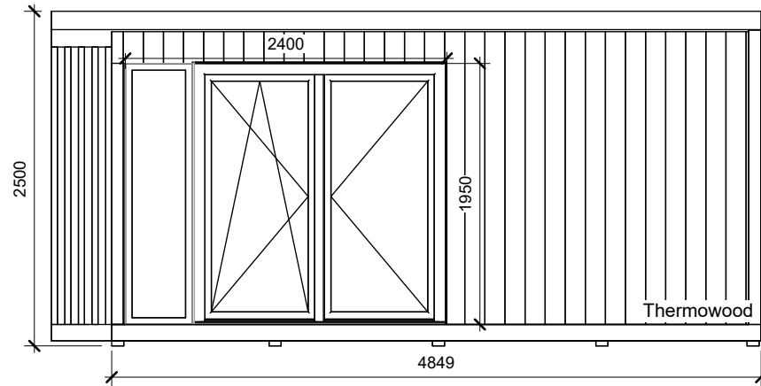
1 Front Elevation 1 : 50
