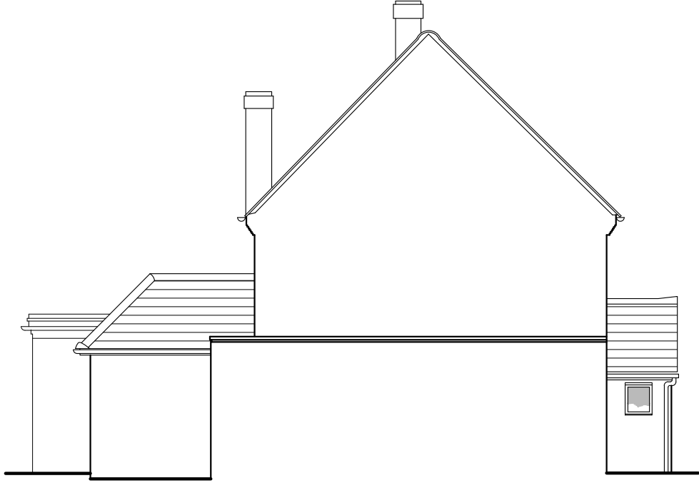
SIDE ELEVATION 1:100
