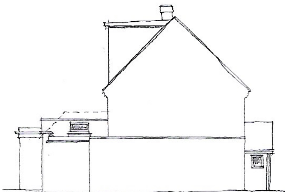
SIDE ELEVATION 1:100
