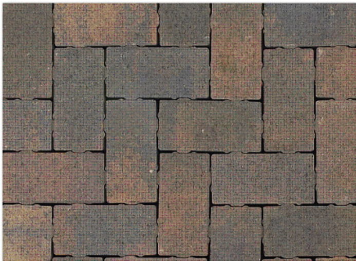
Permeable block paving: to paths and parking bays Tobermore Hydropave or similar approved Colour: Bracken
