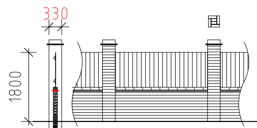
Brick pier/timber fence 1:100
