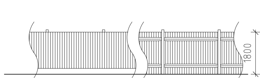
1.8m high Close Board Fence 1:100
