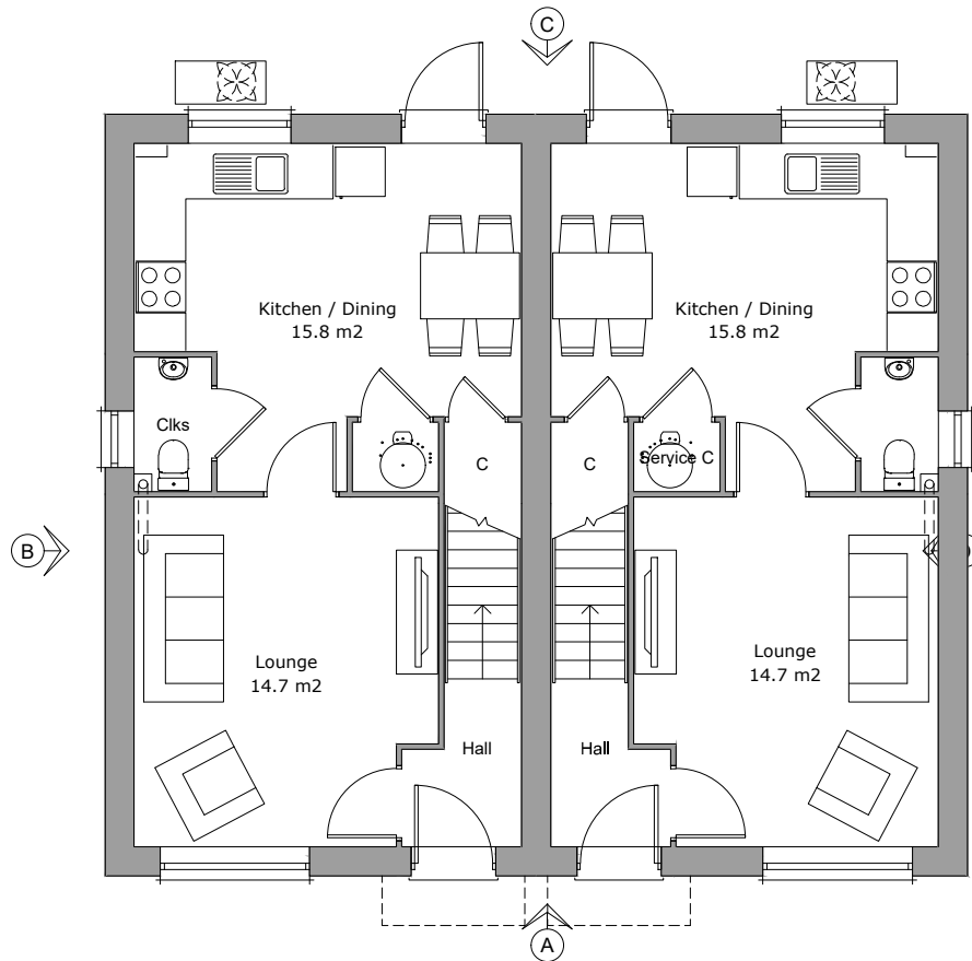
Ground Floor Plan Area 40.0m²
