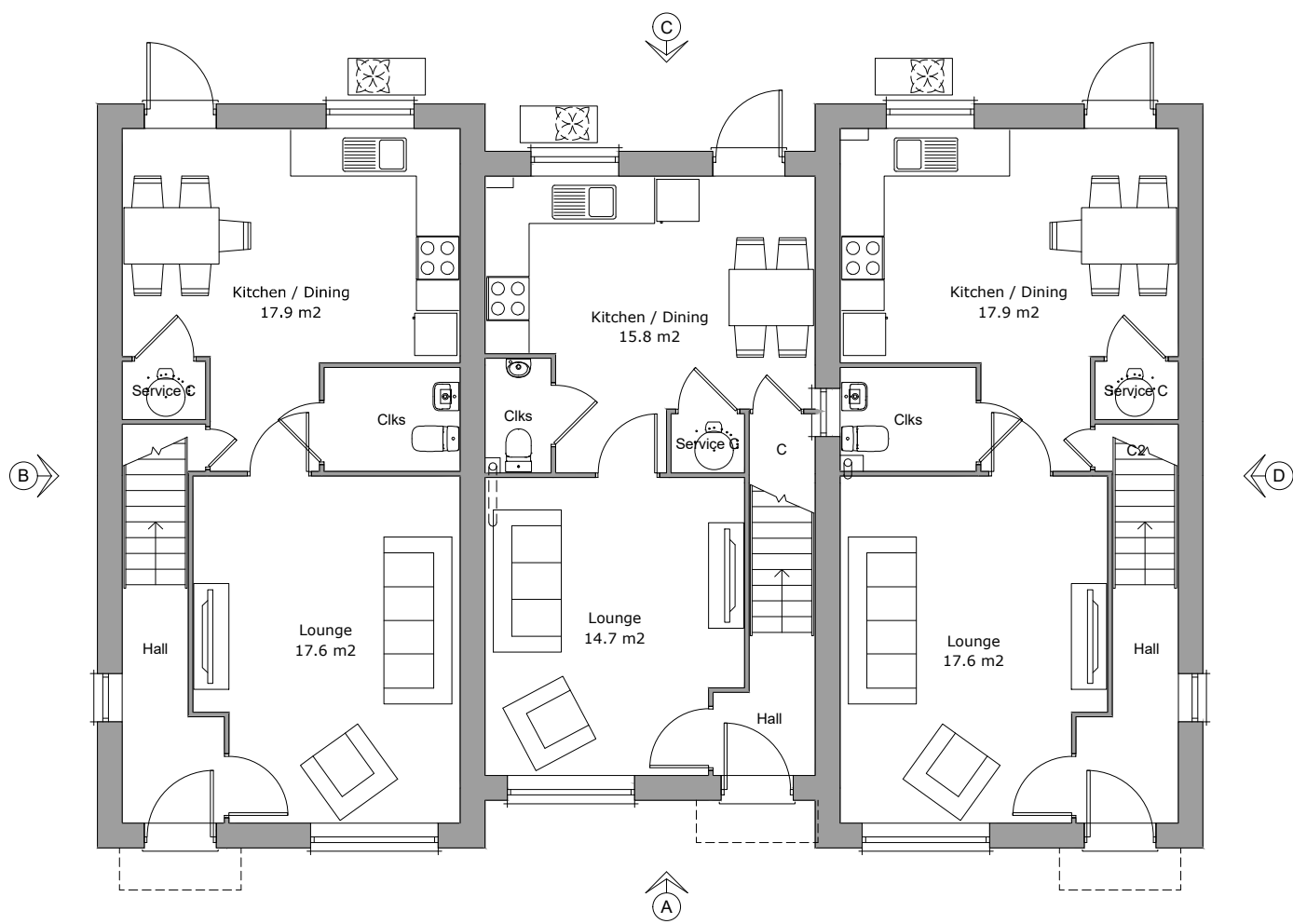
Ground Floor Plan Area 40.0m 2
