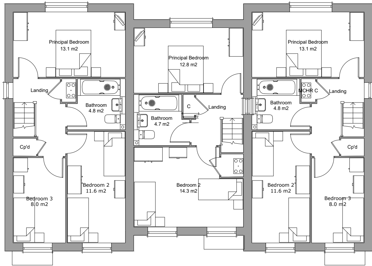
First Floor Plan Area 40.0m 2
