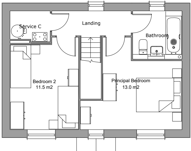
First Floor Plan Area 40.0m²
