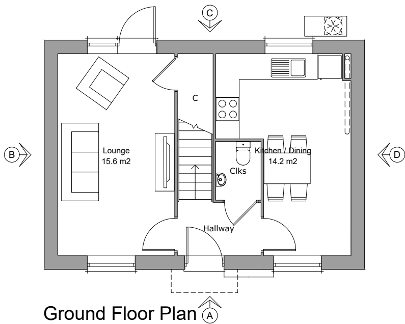
Ground Floor Plan Area 40.0m²
