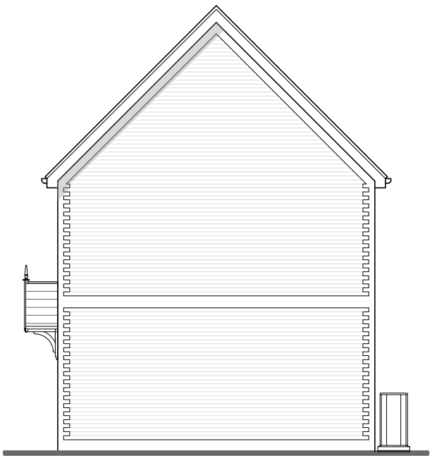
Elevation D
