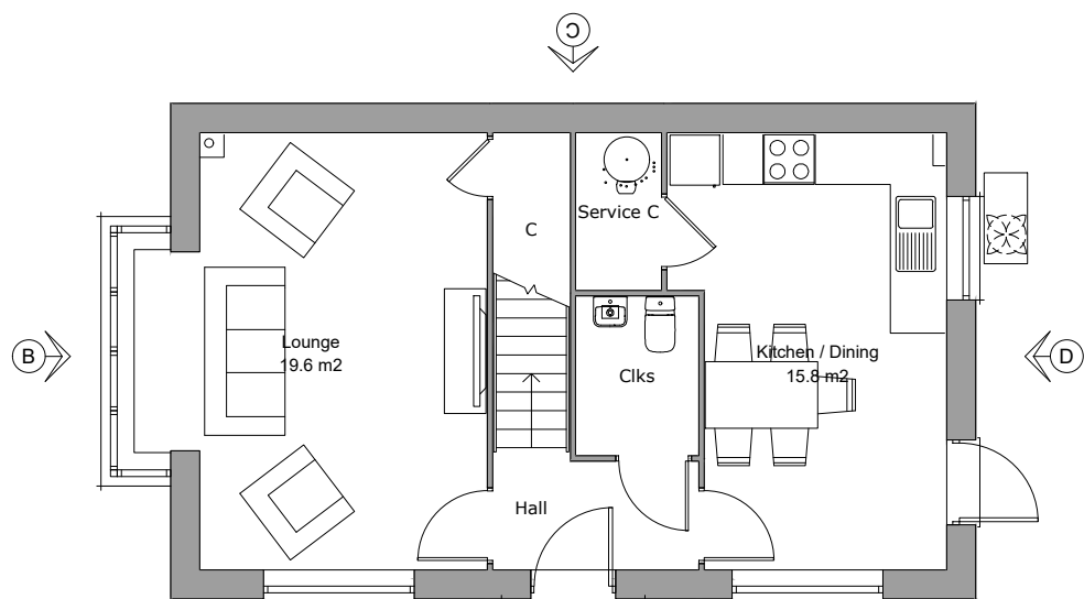
Ground Floor Plan Area 49.0m²
