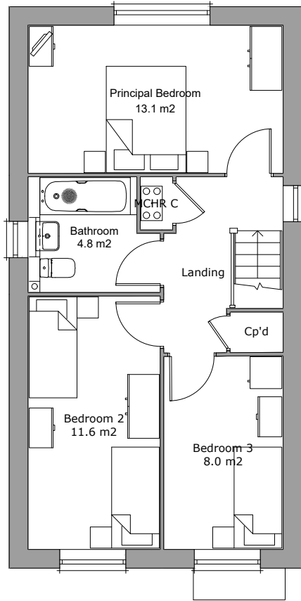
First Floor Plan Area 47.4m²
