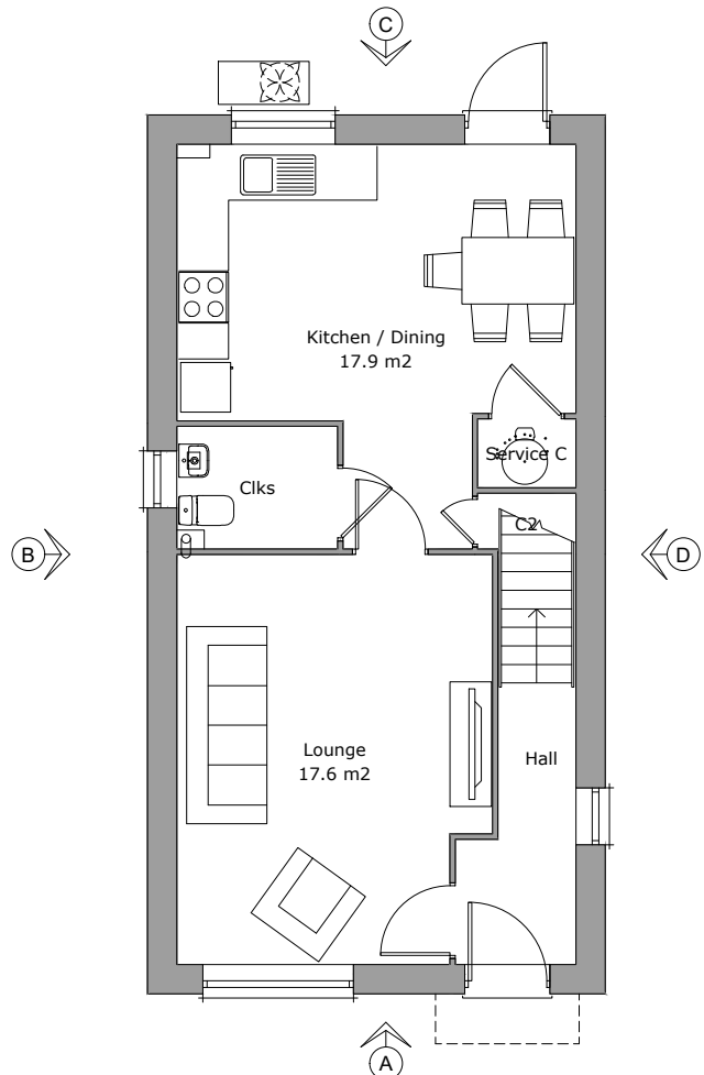
Ground Floor Plan Area 47.4m²
