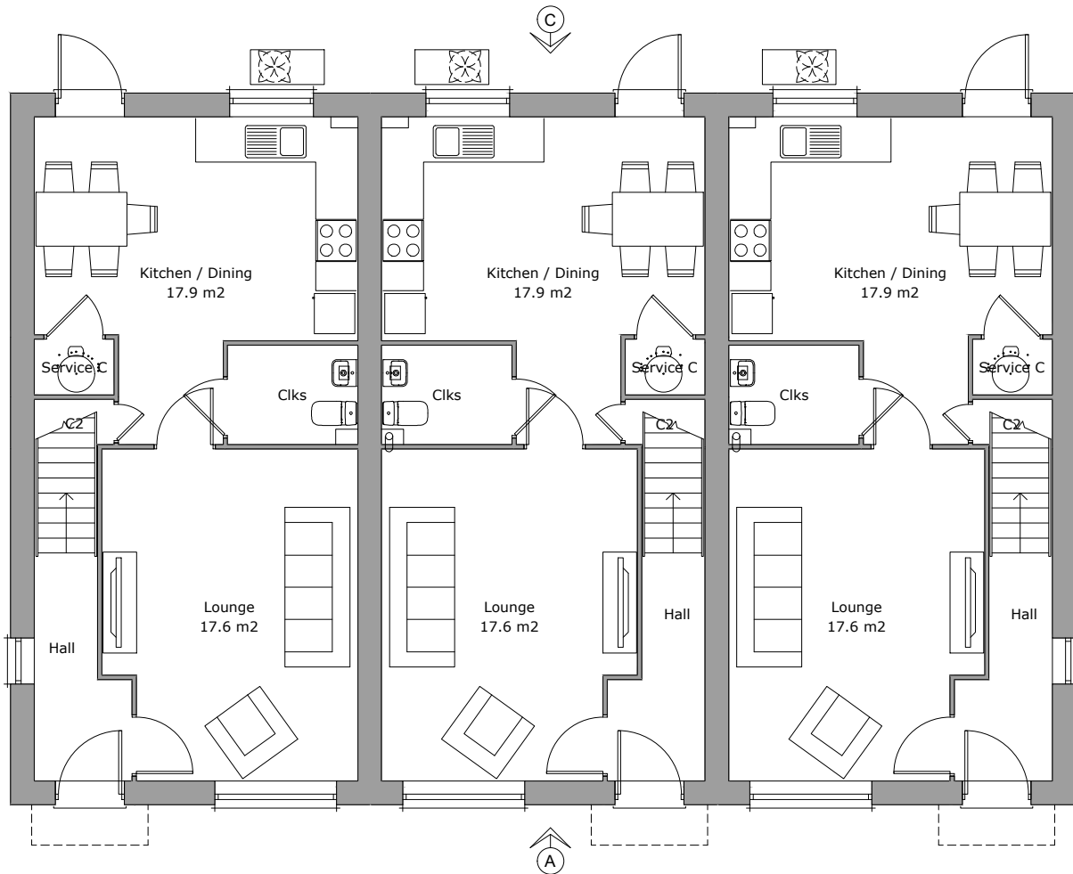
Ground Floor Plan Area 47.4m²
