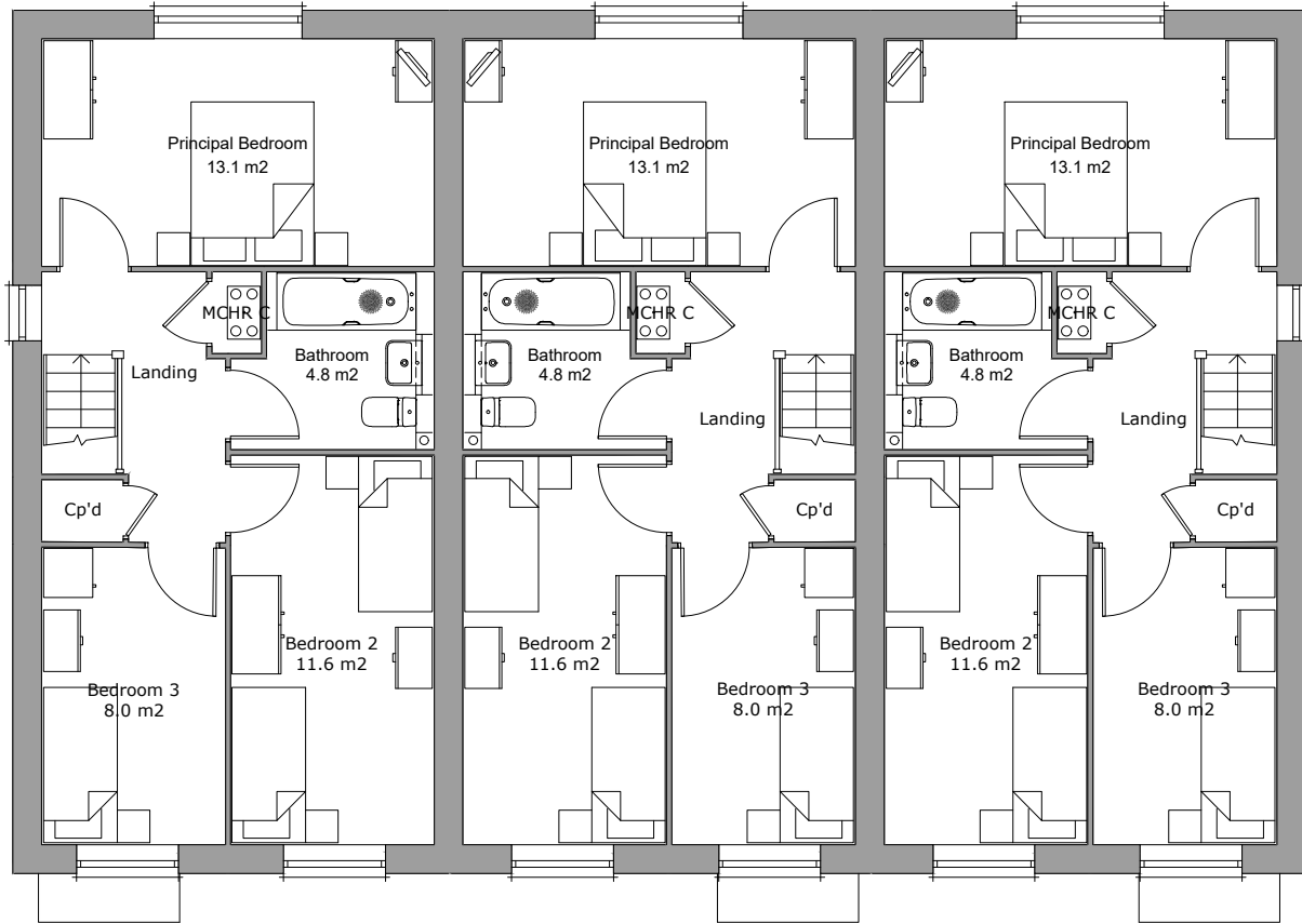
First Floor Plan Area 47.4m²
