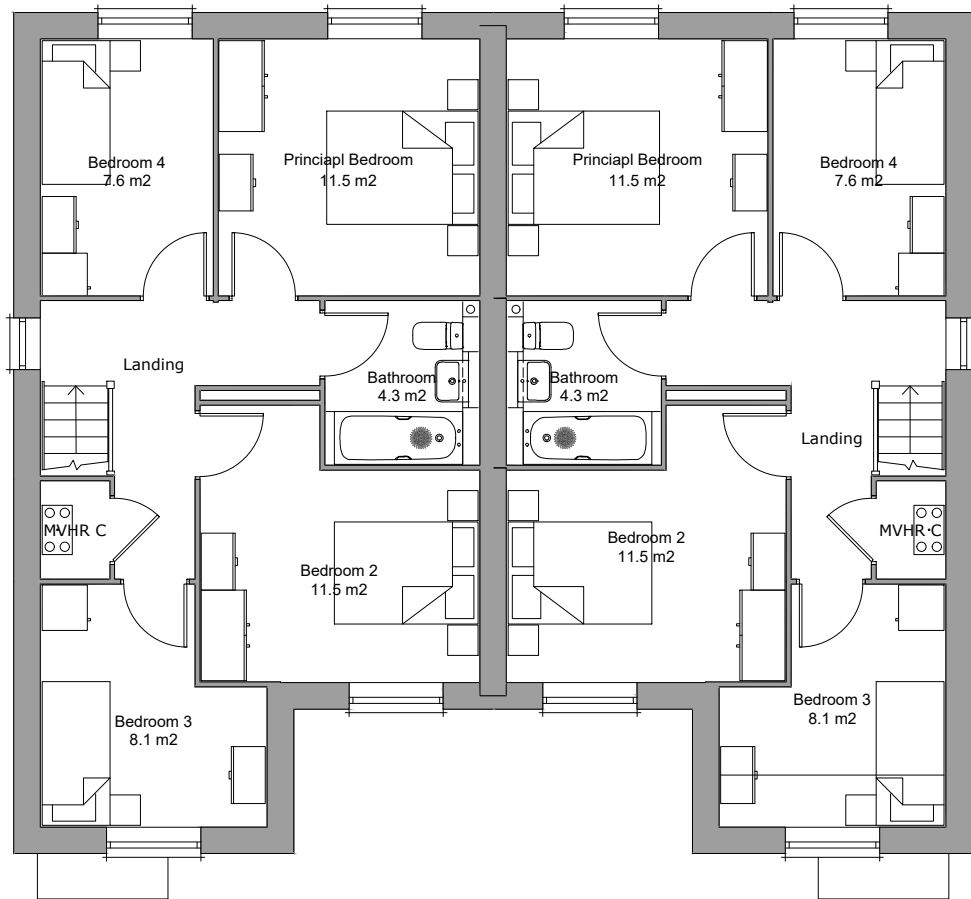
First Floor Plan Area 55.3m²
