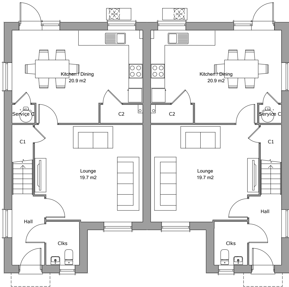
Ground Floor Plan Area 55.3m²
