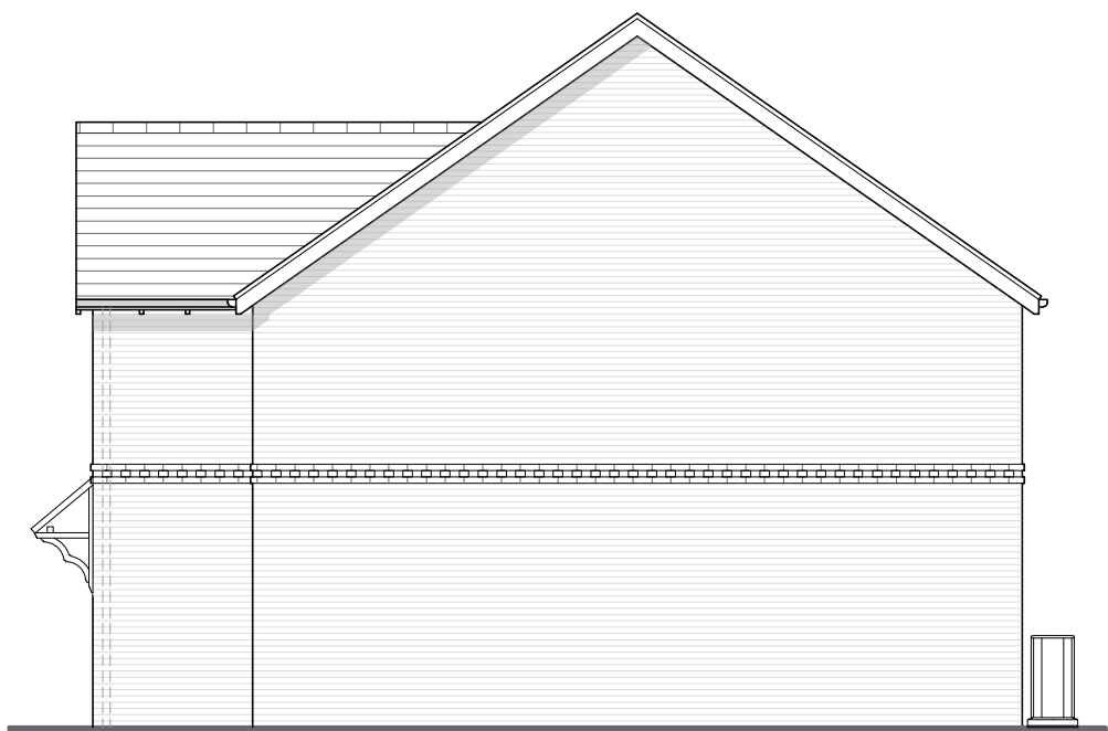
Elevation D
