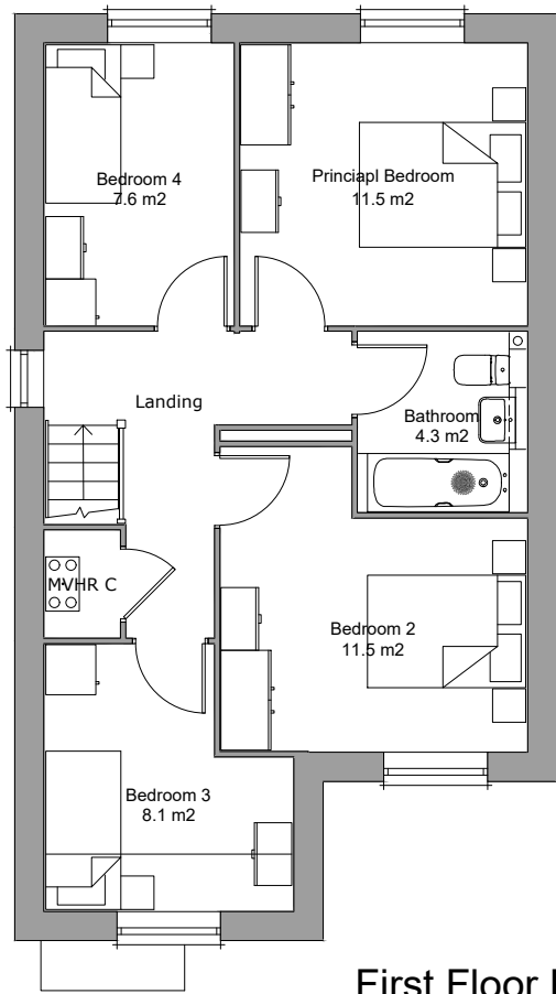
First Floor Plan Area 55.3m²
