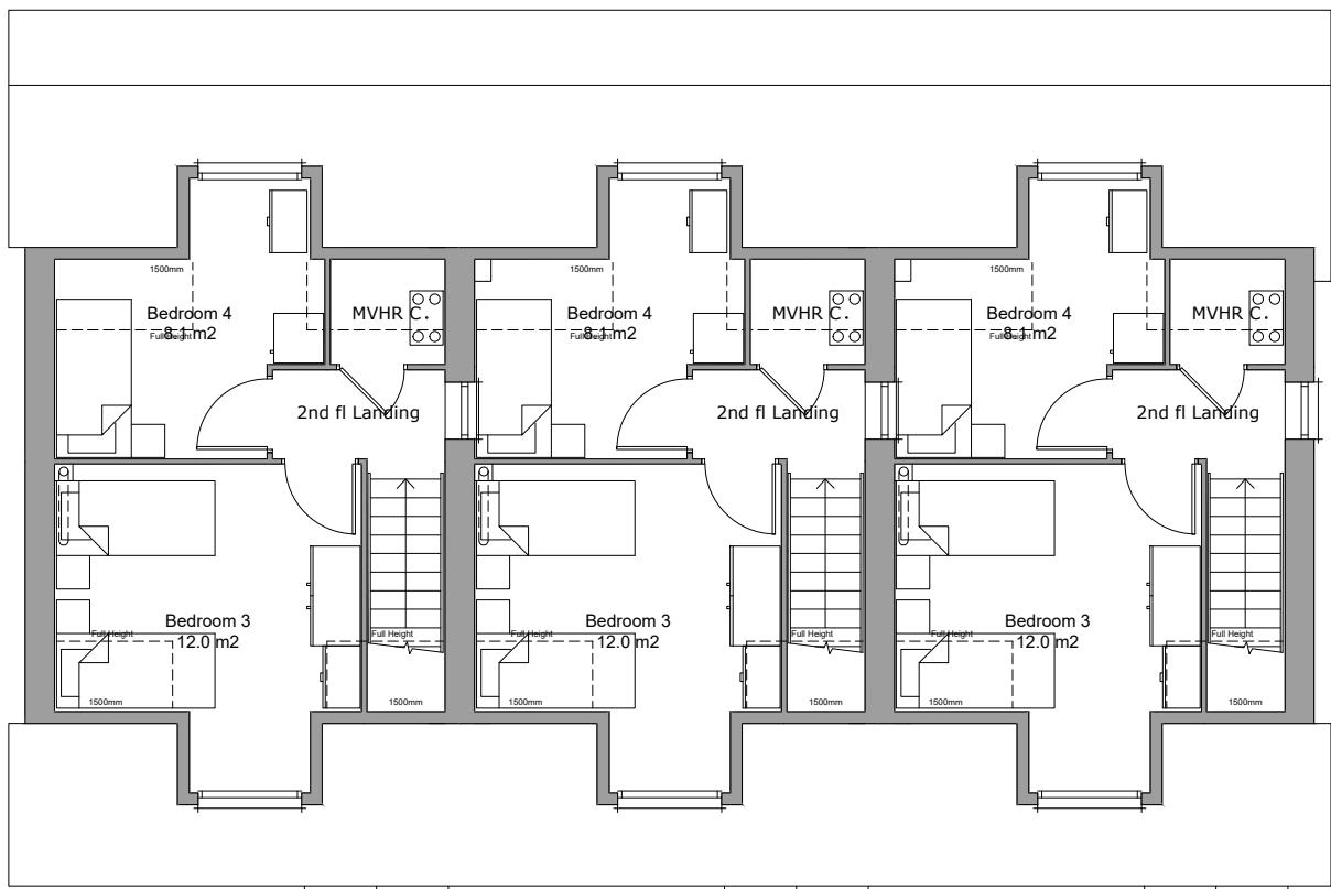
Second Floor Plan Area 23.2m²
