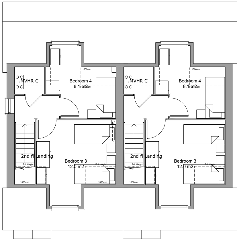
Second Floor Plan Area 23.2m²
