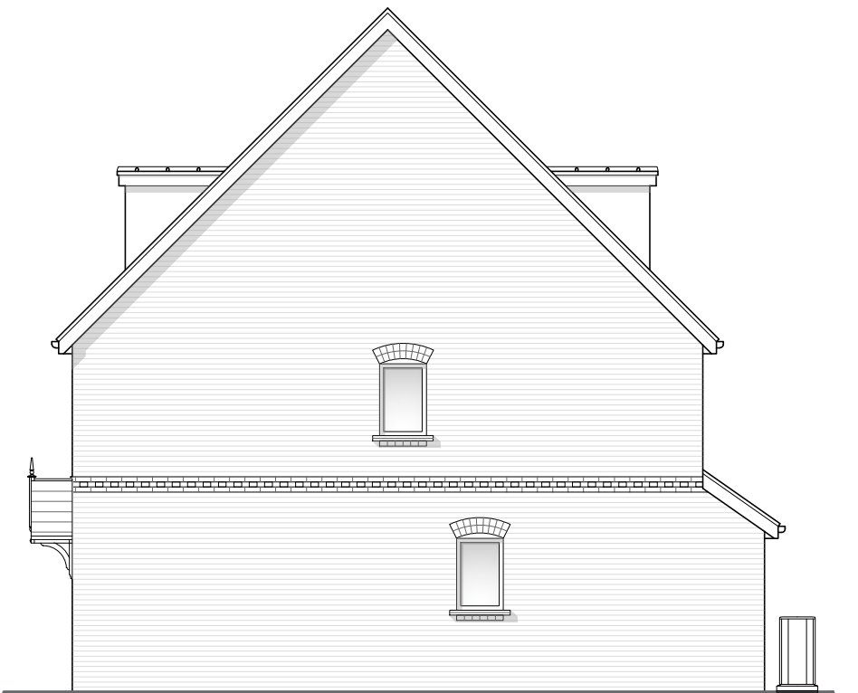
Elevation D
