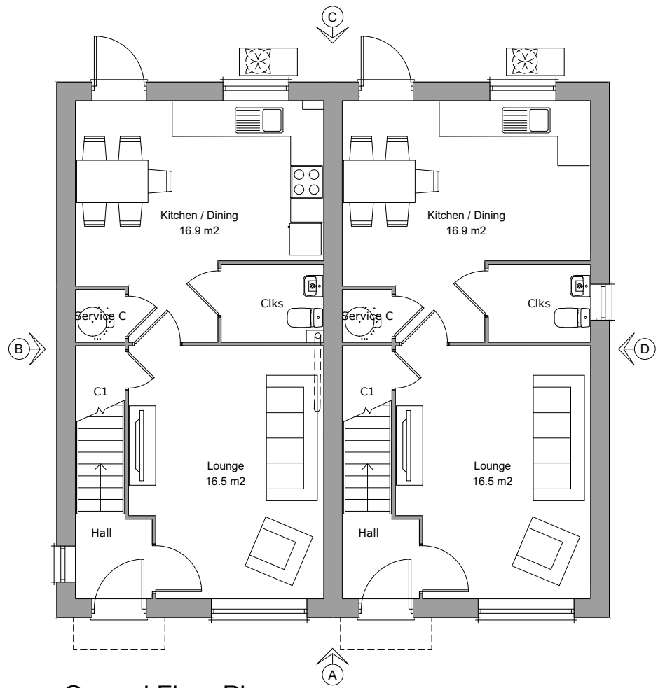
Ground Floor Plan Area 44.2m²
