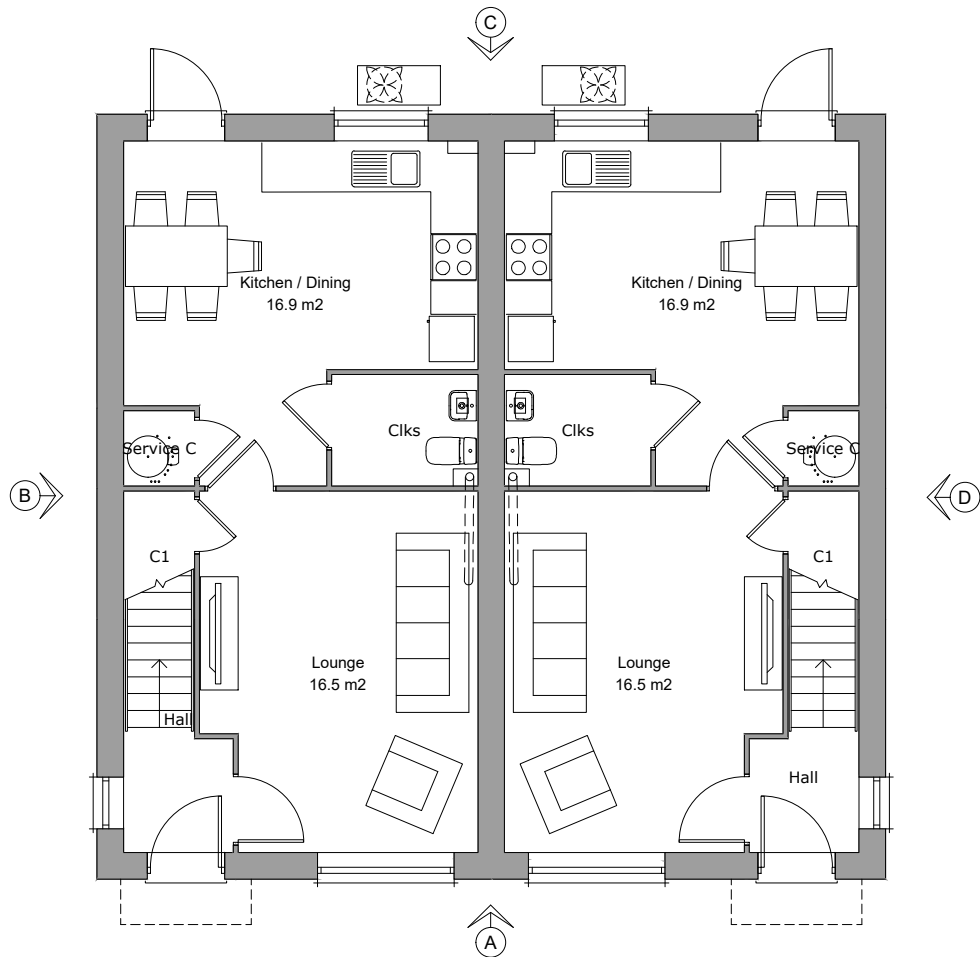
Ground Floor Plan Area 44.2m²
