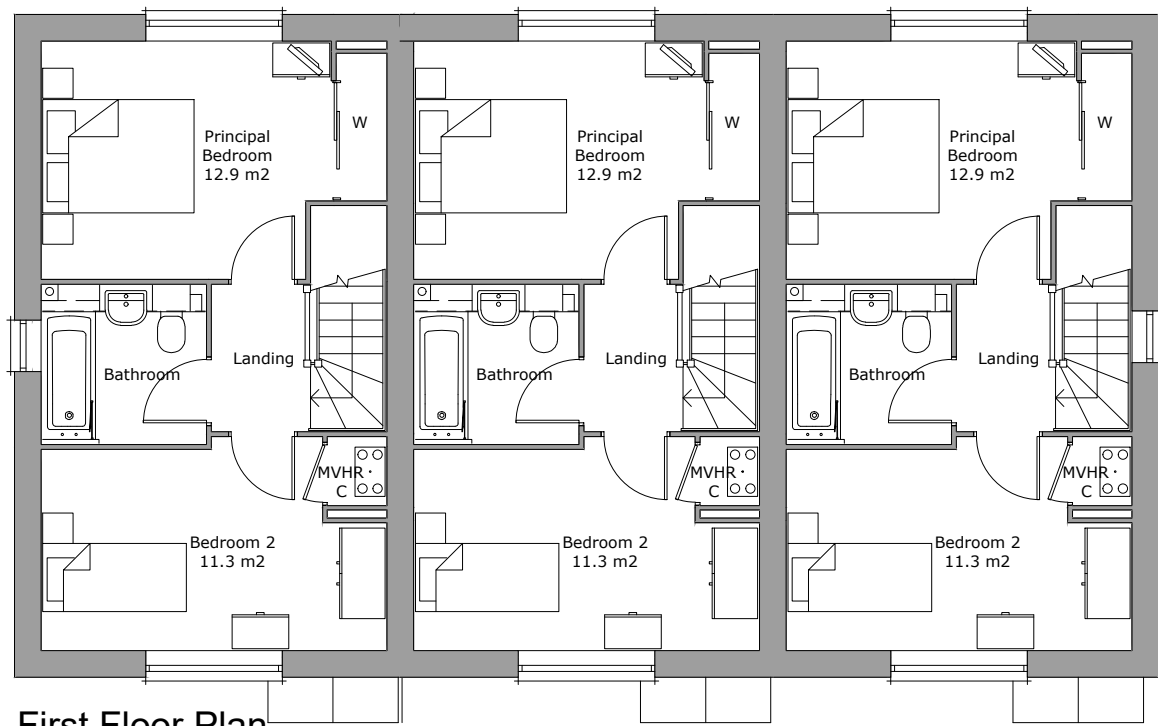
First Floor Plan Area 36.9m²
