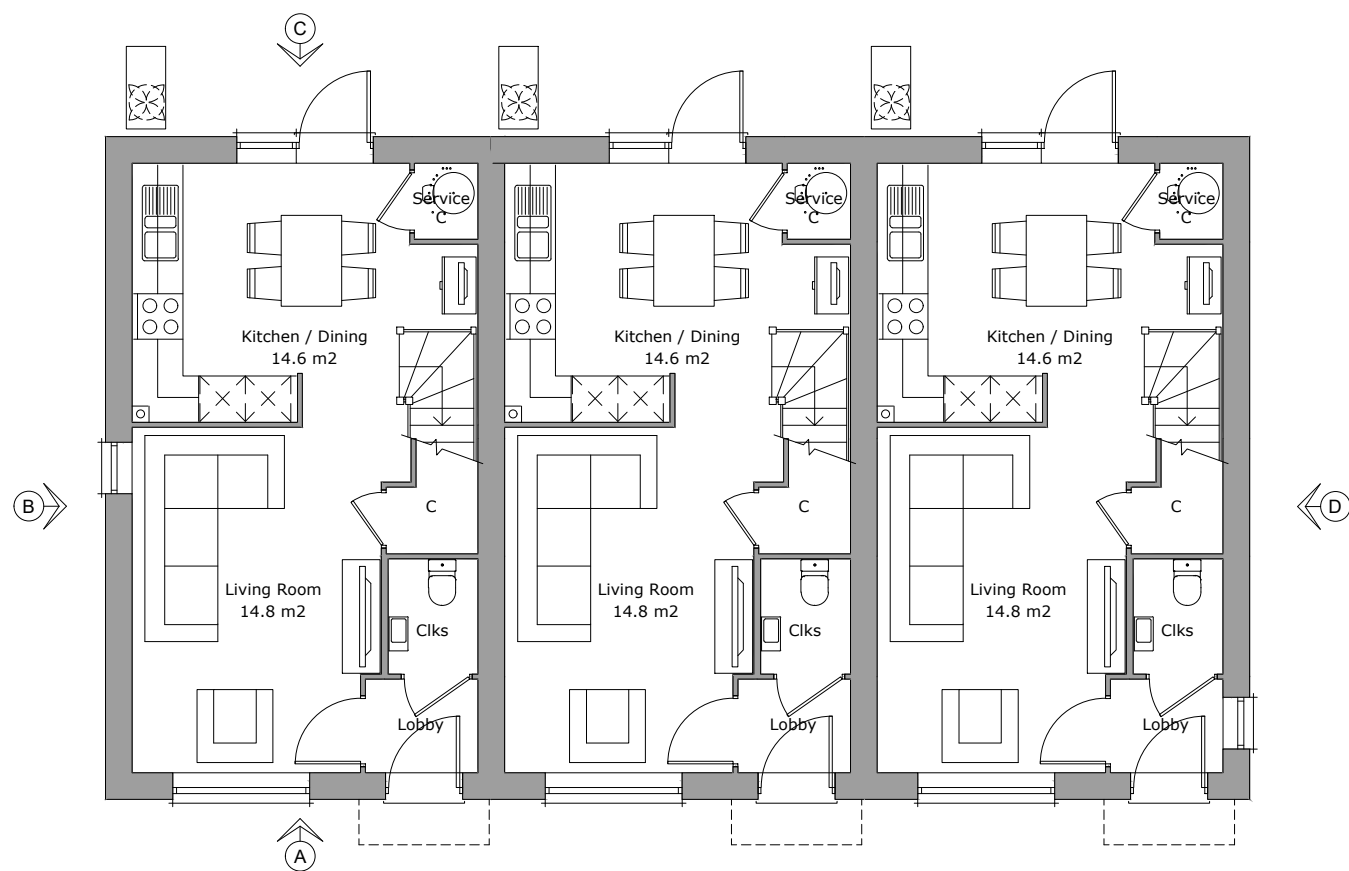
Ground Floor Plan Area 36.9m²
