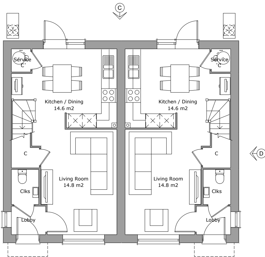
Ground Floor Plan Area 36.9m²
