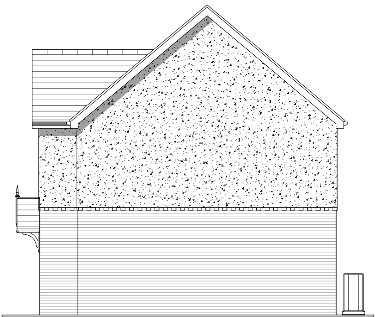
Elevation D
