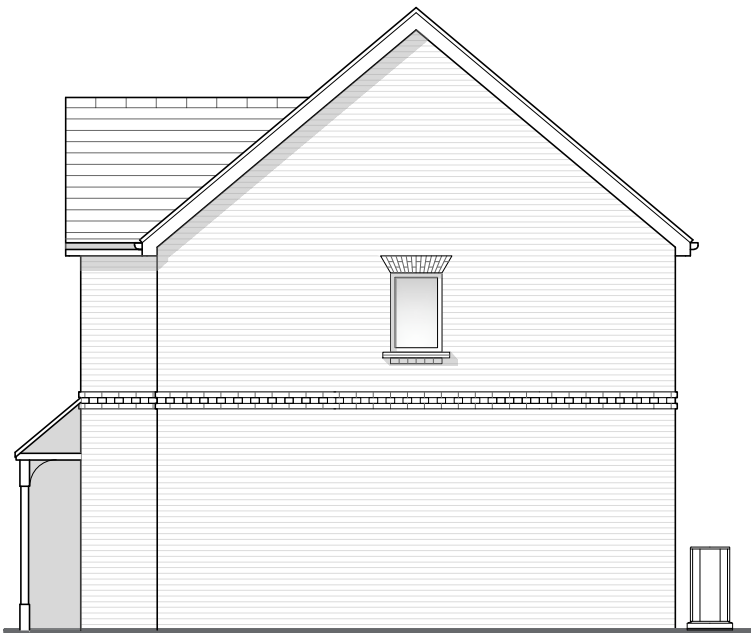
Elevation D
