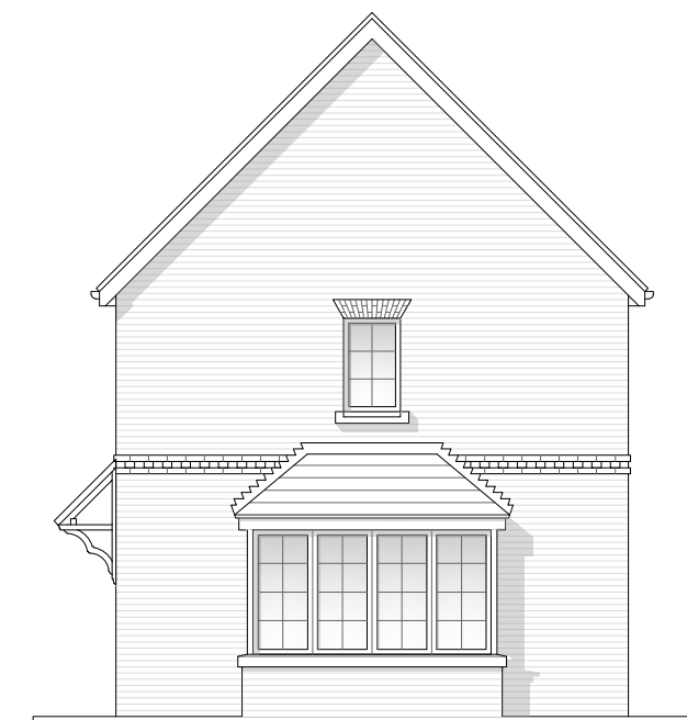
Elevation D
