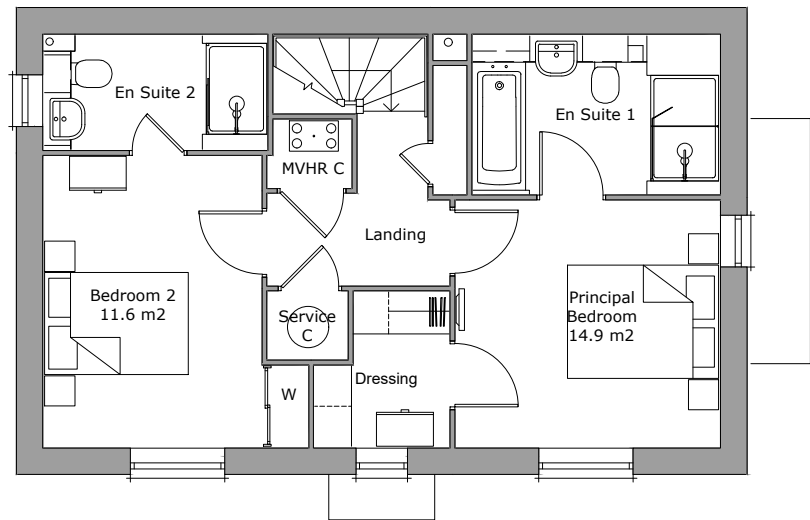
First Floor Plan Area 49.1m 2
