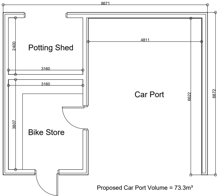
02 PROPOSED FLOOR PLAN 1:100
