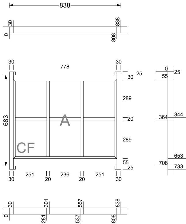
S15 Screen Casement Fixed
