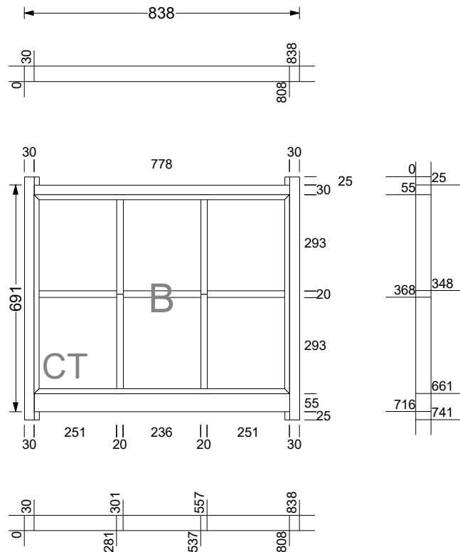
S15 Screen Casement Bottom Sash Sliding
