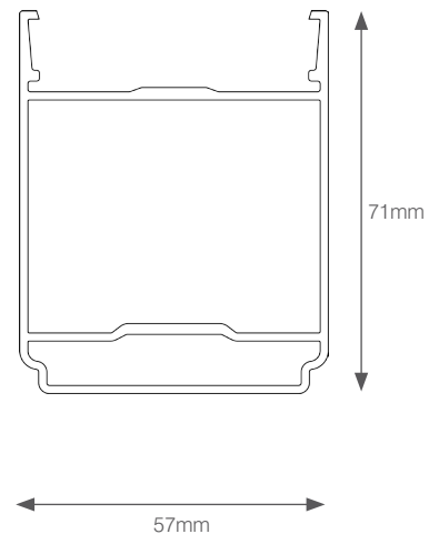
RAFTER BODY KLP-03
