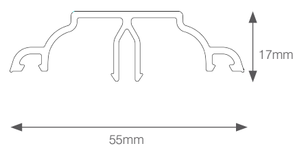
RAFTER TOP CAP KLP-08
