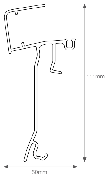
GLASS RETAINER KLP-04
