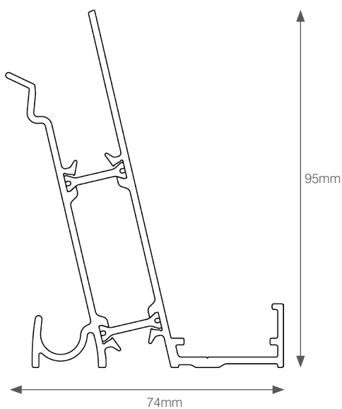
EAVES BEAM KLP-05
