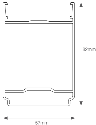
HIP BODY KLP-02
