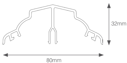
RIDGE TOP CAP KLP-06
