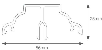
HIP TOP CAP KLP-07
