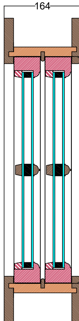
Section through head
