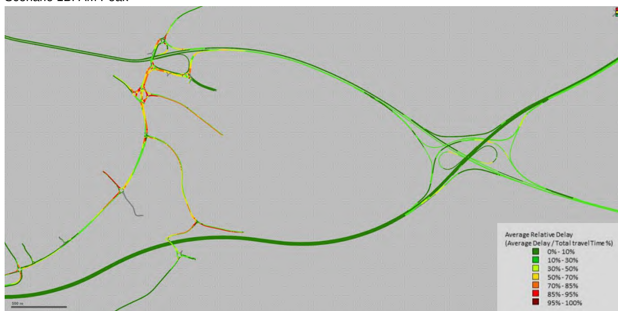
Figure 78: Winnersh and M4 J10. VISSIM Model. Delay Heatmaps. AM Peak
