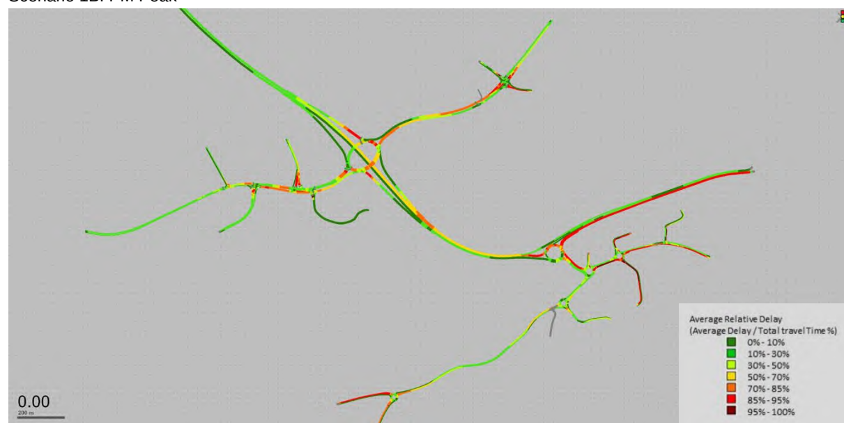
Figure 81: Coppid Beech and Berkshire Way. VISSIM Model. Delay Heatmaps. PM Peak
