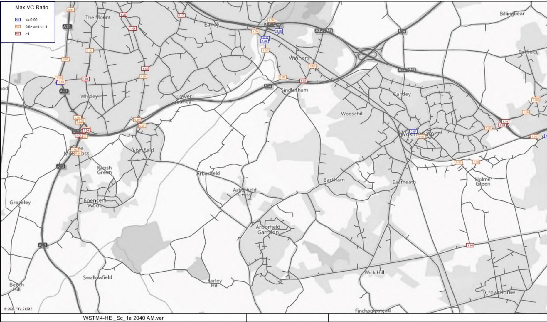
Figure 69: WSTM4. V/C Ratio for the Worst Performing Turn – 2040 Scenario 1A. AM Peak
