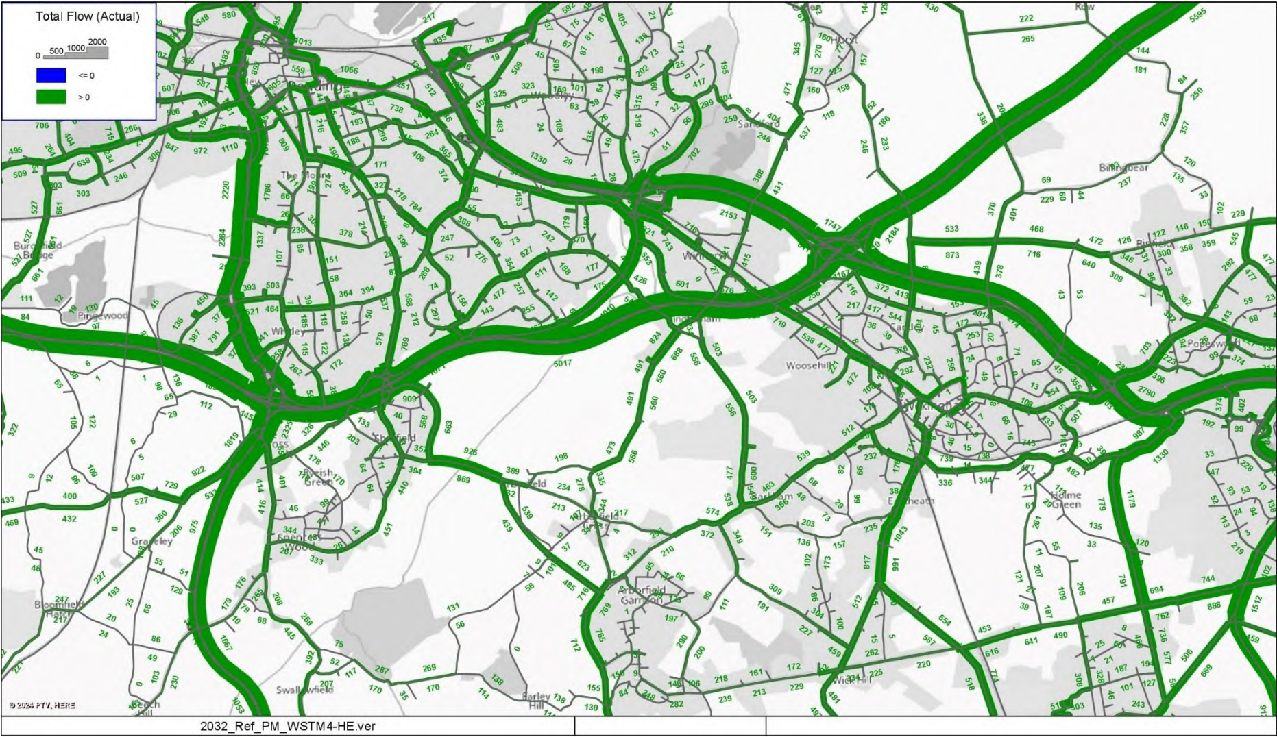
Figure 15: WSTM4. Actual Flows, vehicles – 2032 Reference Case. PM Peak
