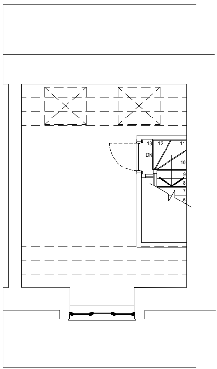
PROPOSED LOFT PLAN
