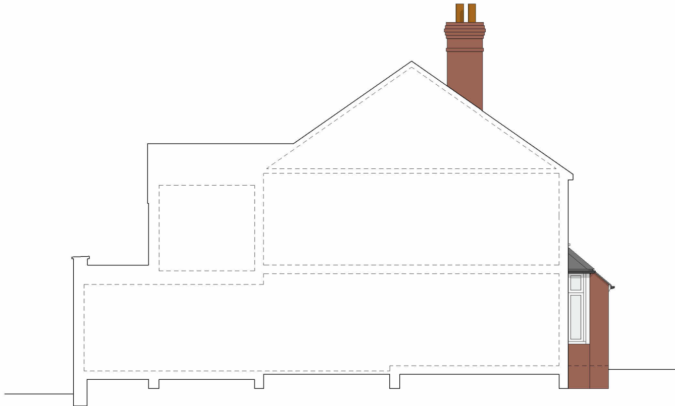
3 Proposed West Elevation A2.01 1 : 100
