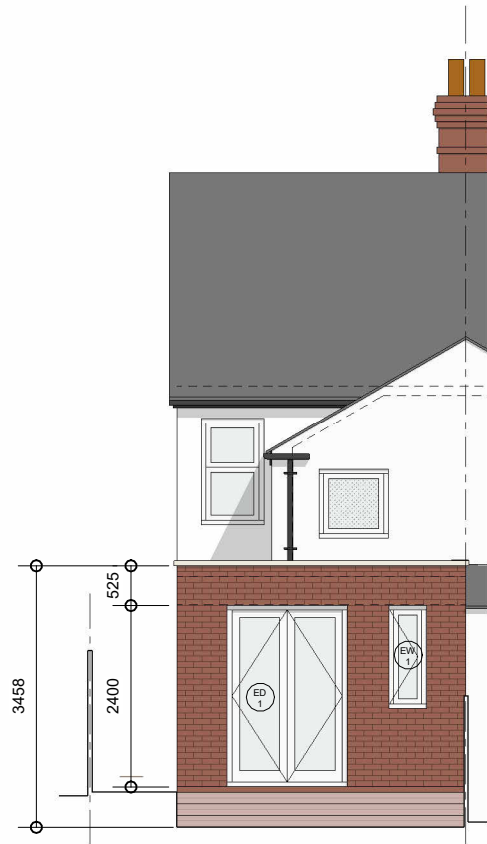
1 Proposed Rear/ South Elevation A2.01 1 : 100
